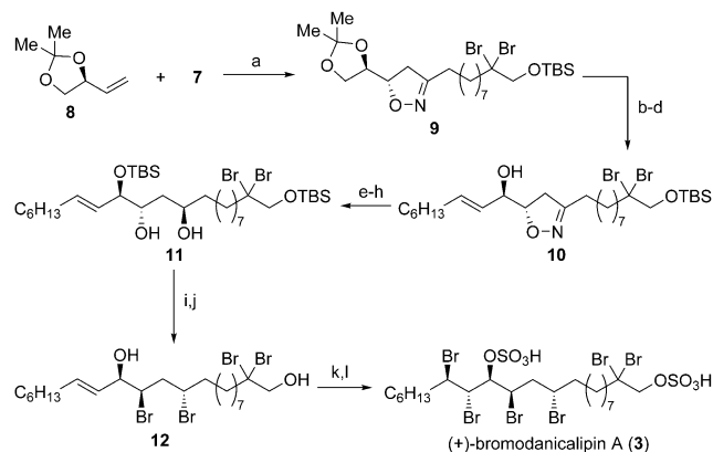
Scheme 2. Reagents and conditions: a) 8 (1.4 equiv), NaOCl (13% in H 2 O, 3.7 equiv), CH 2 Cl 2 , 0 °C to RT, 89%, d.r. = 79:21; b) H 3 [P(W 3 O 10 ) 4 ·(H 2 O) 24 ] (3 mol %), MeCN/H 2 O (10:1), RT; c) NaIO 4 (1.3 equiv), THF/pH 7 buffer (1:1), 0 °C to RT, 75% over 2 steps; d) oct-1-yne (1.5 equiv), Cp 2 Zr(H)Cl (1.2 equiv), Me 2 Zn (1.2 equiv), CH 2 Cl 2 , −78 °C to RT, 85%, d.r. = 76:24, 95% ee ; e) TBSOTf (1.3 equiv), Et 3 N (1.5 equiv), CH 2 Cl 2 , 0 °C; f) Mo(CO) 6 (1.2 equiv), MeCN/H 2 O (10:1), 90 °C; g) i PrCHO (11 equiv), Sml 2 (0.09 M in THF, 30 mol %), THF, −30 °C; h) ( i Bu) 2 AlH (3.0 equiv), CH 2 Cl 2 , −78 °C, 67% over 4 steps; i) CBr 4 (4.9 equiv), PPh 3 (5.4 equiv), pyridine (13 equiv), CH 2 Cl 2 , RT, 45%; j) HF-pyridine (33 equiv), THF, 0 °C to RT, 99%; k) PhNMe 3 Br 3 (1.4 equiv), CH 2 Cl 2 , 0 °C to RT, 99%, d.r. = 90:10; l) SO 3 ·pyridine (4.1 equiv), THF, RT, 99%. Cp = cyclopentadienyl, TBS = tert -butyldimethylsilyl, Tf = trifluoromethanesulfonyl.
