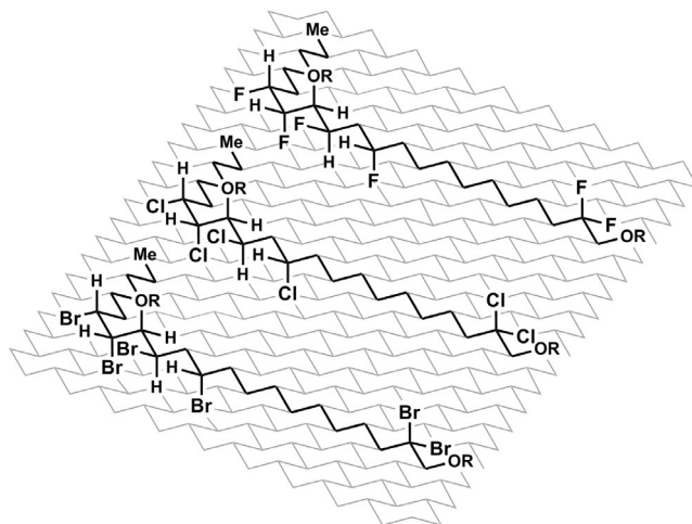
Figure 2. Ground-state conformation in solution (R = H) determined for C11 to C16 by J-based configuration analysis (for numbering see Figure 1).
