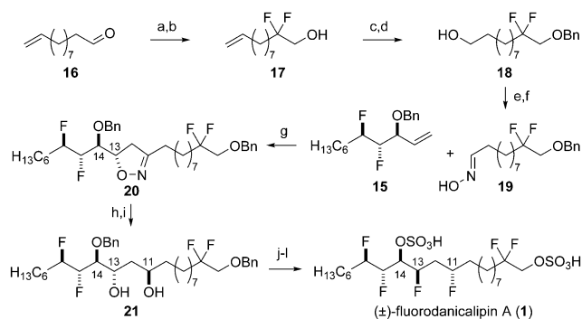
Scheme 4. Reagents and conditions: a) DL-(±)-proline (2.0 equiv), (PhSO 2 ) 2 NF (2.5 equiv), THF, RT, 48 h; b) NaBH 4 (3.0 equiv), CH 2 Cl 2 /EtOH (3:2), RT, 2 h, 86% for 2 steps; c) BnBr (1.5 equiv), NaH (1.5 equiv), n Bu 4 NI (10 mol%), THF, −15 °C to RT, 2.5 h, 84%; d) BH 3 ·THF (0.5 equiv), THF, 0 °C to RT, 5 h; then 3.0 M aq. NaOH (1.1 equiv), H 2 O 2 (3.1 equiv), 0 °C to RT, 1.5 h, 99%; e) DMP (1.9 equiv), t BuOH (1.9 equiv), CH 2 Cl 2 , RT, 0.5 h, 71%; f) Et 3 N (1.2 equiv), MeOH, RT; then HONH 2 ·HCl (1.1 equiv), 20 min, 99%, E/Z = 6:4; g) 15 (1.0 equiv), NaOCl, 13% in H 2 O (3.0 equiv), CH 2 Cl 2 , syringe pump addition of 19 (1.2 equiv) over 24 h; RT; then RT, 16 h, 62%, d.r. > 95:5; h) Mo(CO) 6 (1.3 equiv), MeCN/H 2 O (10:1), 90 °C, 1.5 h, 84%; i) Me 4 NBH(OAc) 3 (10 equiv), MeCN/AcOH/CH 2 Cl 2 (5.5:2.5:1), 0 °C, 2 h, 88%, d.r. = 87:13; j) (MeOCH 2 CH 2 ) 2 NSF 3 (6 equiv), CH 2 Cl 2 , 0 °C, 1 h; then RT, 24 h; k) Pd/C (15 mol%), H 2 (1 atm), MeOH, RT, 6 h, 42% for 2 steps; l) SO 3 ·pyridine (4.0 equiv), THF, RT, 1.5 h, 93%. DMP = Dess–Martin periodinane.
